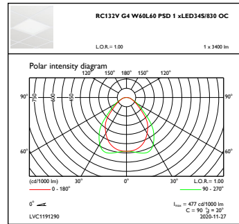
OFPC1_RC132VG4W60L60PSD1xLED34S830OC
